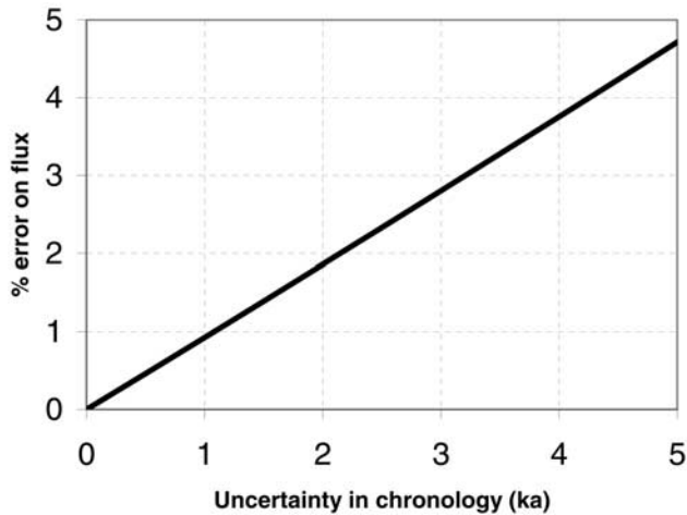
Figure 4. Error on ^{230}\text{Th} normalized flux engendered by errors in core chronology.
