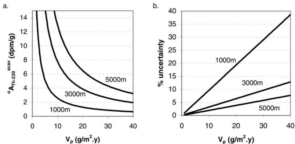
Figure 5. (a) Relationship between the scavenged ^{230}\text{Th} activity ( {}^0A_{\text{Th-230}}^{\text{scav}} ) and vertical settling fluxes of particles ( F_V ) at three different depths. {}^0A_{\text{Th-230}}^{\text{scav}} was calculated according to equation (9): {}^0A_{\text{Th-230}}^{\text{scav}} = \beta_{230} Z/F_V . (b) Uncertainty on estimating vertical settling flux ( F_V ) by ^{230}\text{Th} normalization when {}^0A_{\text{Th-230}}^{\text{scav}} has an uncertainty of 0.25 dpm \text{g}^{-1} .
